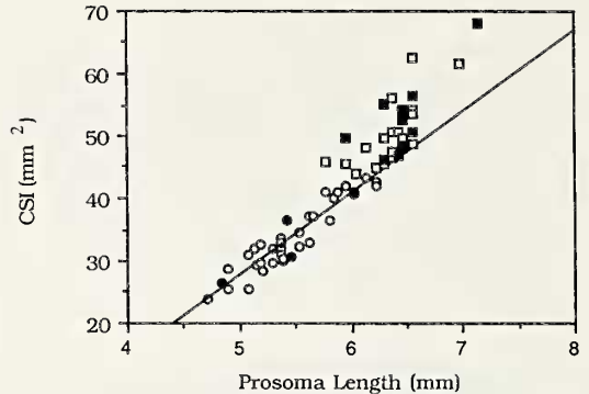
Figure 2.—Relationship between chela-size index (CSI = length of chela \times width) and prosoma length in adult males. Data have been separated into two instars (see text), sixth (circles) and seventh (squares). Regression line fits the relationship in the sixth instar: seventh instar males have allometrically larger chelae. Regression line: y = 12.9x - 37.1 , R^2 = 0.88 . Males known to have deposited a spermatophore (filled symbols) occur in both instars.
